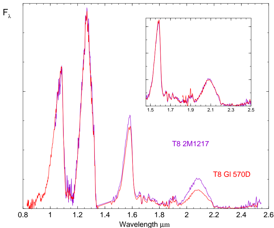
Figure 4. Observed relative flux distributions of two T8 dwarfs, from Geballe et al. 2001a; inset shows different scalings, see text.
