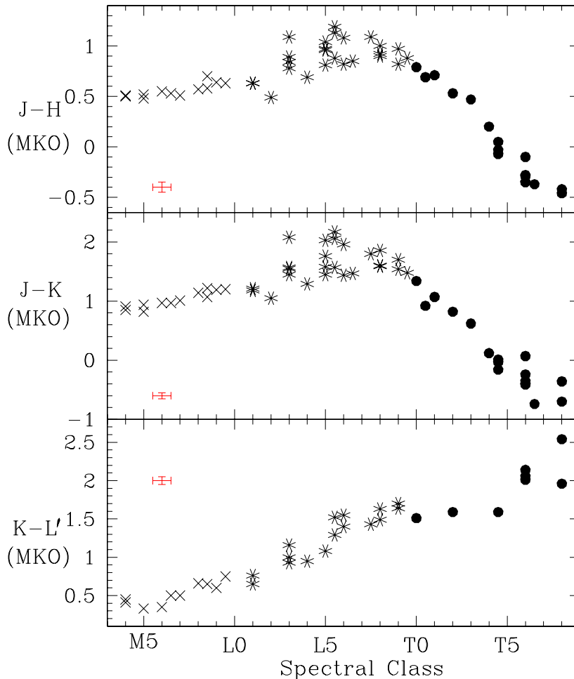
Figure 1. J - H , J - K and K - L' against spectral type for M dwarfs (crosses), L dwarfs (asterisks) and T dwarfs (filled circles); photometry from Leggett et al. 2001, spectral classification by Geballe et al. 2001a. Typical error bars are shown in red.
