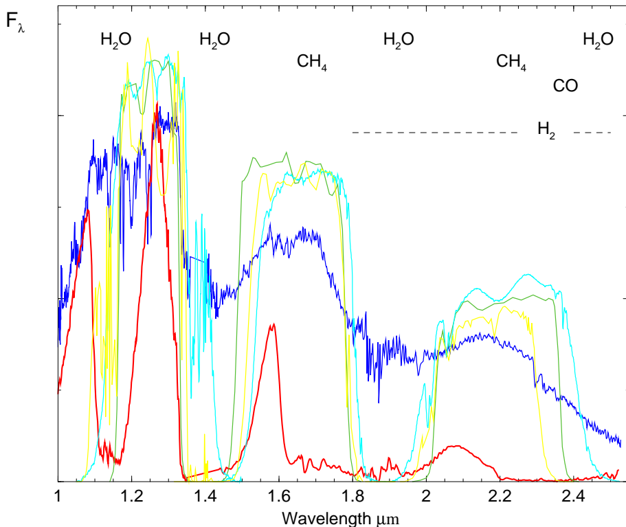
Figure 2. Observed spectra of an L1 dwarf (2MASS J0746+20, Reid et al. 2001, blue line) and a T8 dwarf (Gl 570D, Geballe et al. 2001b, red line). J, H, K filter profiles are overlaid from the MKO (green), UKIRT (cyan) and 2MASS (yellow) photometric systems.
