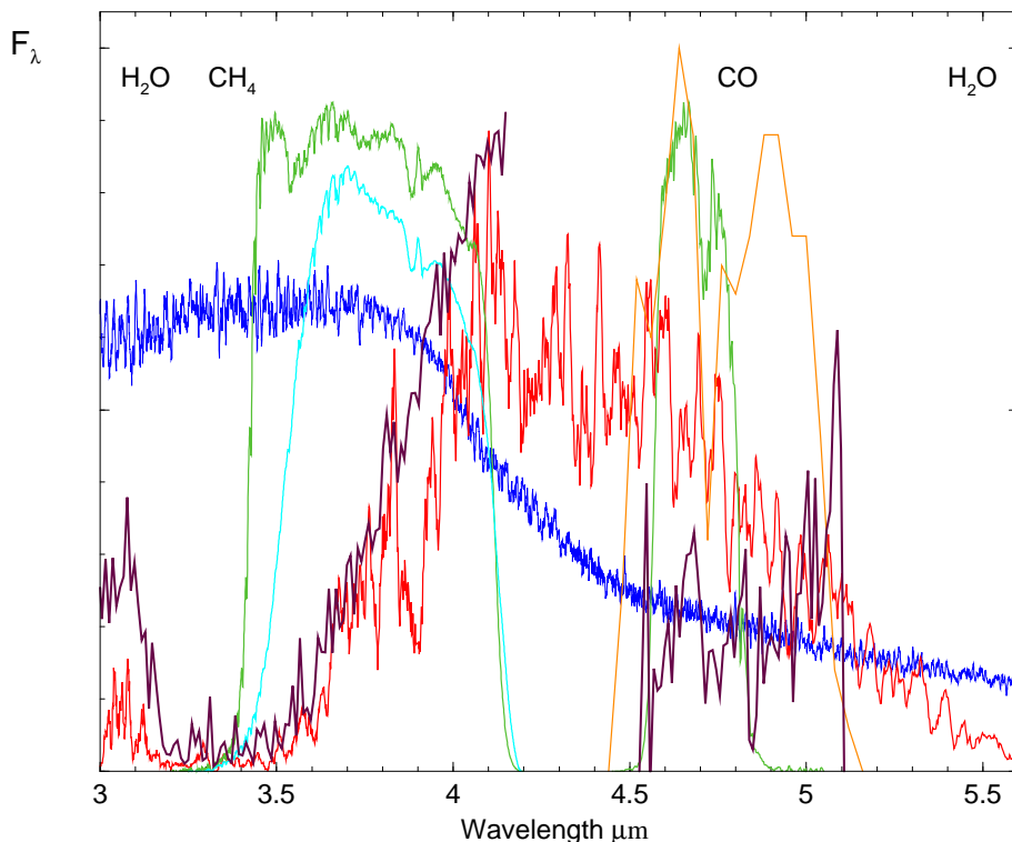
Figure 5. Calculated spectra for an L dwarf type atmosphere with T_{\text{eff}} = 2000 K (Allard et al. 2001, blue line), and for a T dwarf type atmosphere with T_{\text{eff}} = 800 K (model by D. Saumon and M. Marley, as presented in Geballe et al. 2001b, red line). Also shown is an observed spectrum for the T6 dwarf Gl 229B (Oppenheimer et al. 1998 and Noll et al. 1997, maroon). UKIRT (cyan) L' , MKO (green) L' and M' , and AAO (orange) M filter profiles are overlaid.
