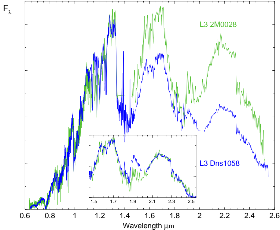
Figure 3. Observed relative flux distributions of two L3 dwarfs, from Geballe et al. 2001a; inset shows different scalings, see text.
