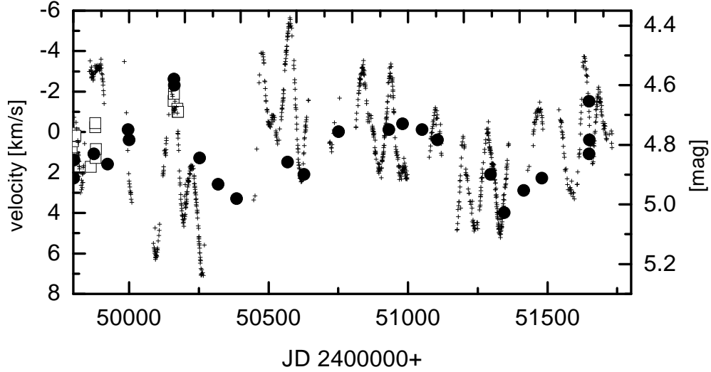
Figure 1. Velocity measurements for g Her compared with its light variations (Percy et al. 2001). Filled circles mark measurements from the current investigation, open boxes denote data from Lebzelter (1999). The velocities have been plotted with the most negative velocity at the top.
