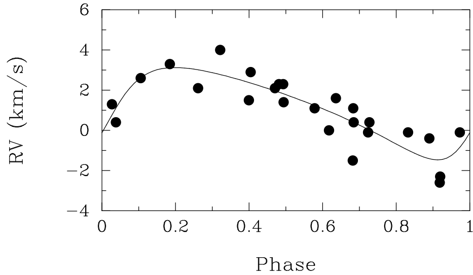
Figure 2. Velocities of g Her phased with a period of 843.7 days. The solid curve is the computed “orbit”.
