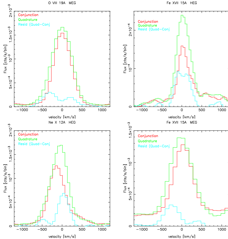
Figure 2. A comparison of line profiles between quadrature (green) and conjunction (red) for wavelengths having the highest spectral resolution. Residuals are shown in light blue.
