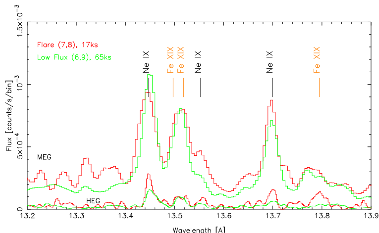
Figure 3. The Ne IX He-like triplet region for both MEG (upper traces), and HEG (lower traces). HEG has higher resolution, but less effective area. The spectra from the flare states are shown in red, and the low-flux states are in green. The forbidden line (13.7 Å) to intercombination line (13.55 Å) ratio is density sensitive.
