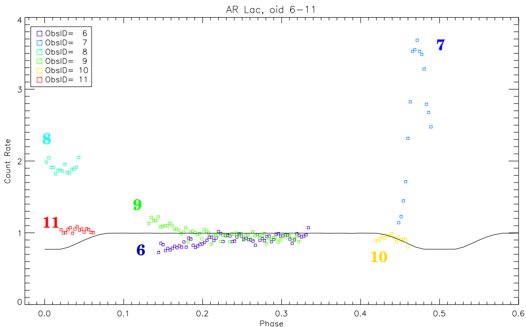
Figure 1. The count-rate is shown against orbital phase. Each observation ID is color coded and labeled. The time-order of ObsIDs is 6, 8, 7, 9, 11, 10. One-sigma uncertainties are slightly larger than the symbol size. The solid line is a simple light curve model assuming uniformly emitting disks of equal intensity. It was arbitrarily placed at a level which suggests that ObsID 10 may show eclipse modulation as the larger K0 IV occults the G2 IV.
