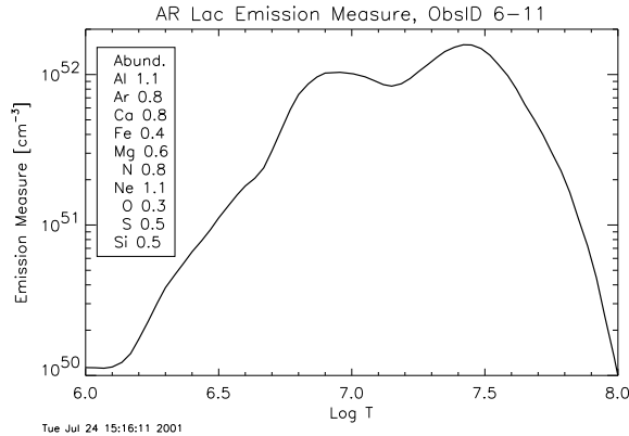
Figure 4. A provisional differential emission measure derived from line fluxes integrated over all observations. This DEM was used to generate the model spectrum shown in Figure 5.
